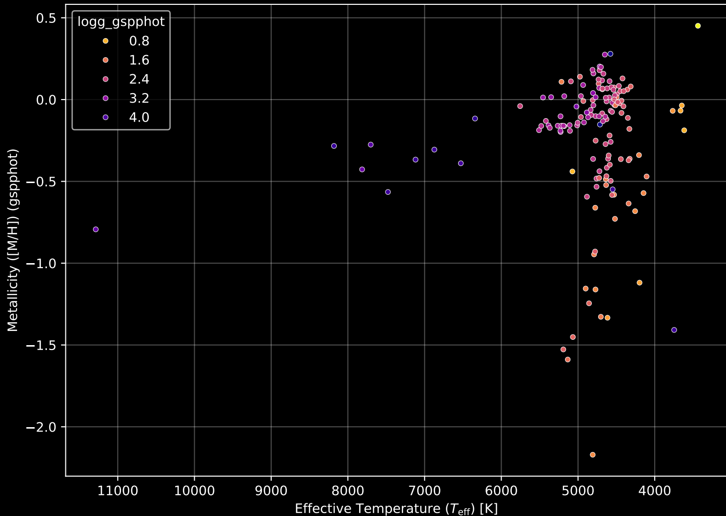
APOGEE DR17 Field: [317+12] Stellar Population Parameters (n= 149)
