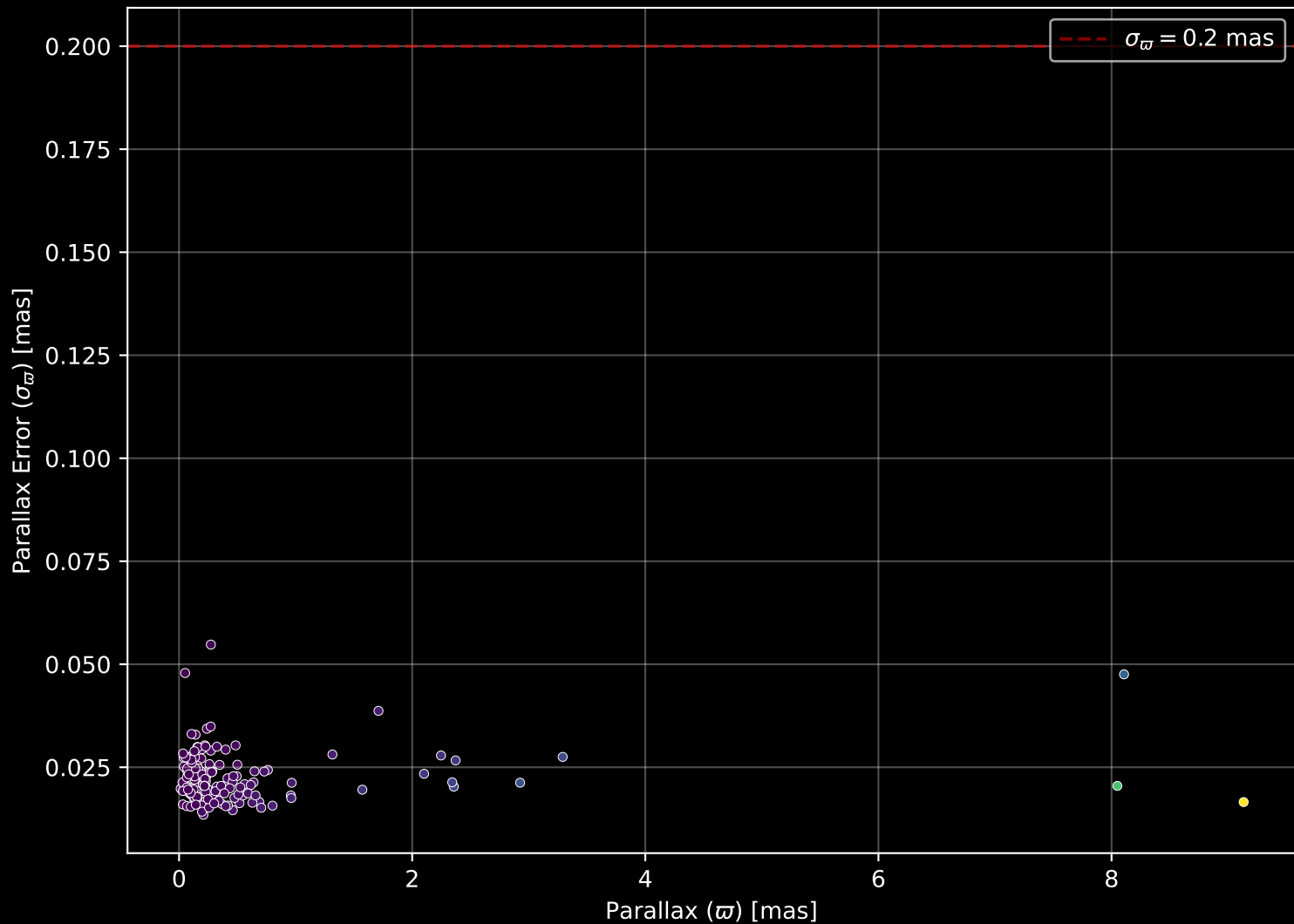
APOGEE DR17 Field: [317+12] Parallax Quality (n= 149)
