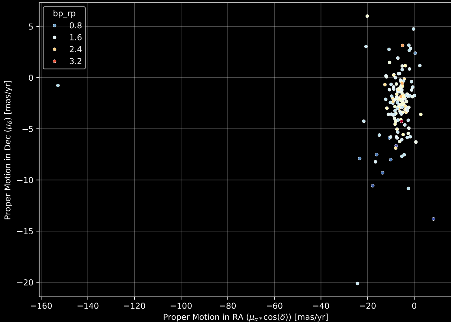
APOGEE DR17 Field: [317+12] Proper Motion Diagram (n= 149)
