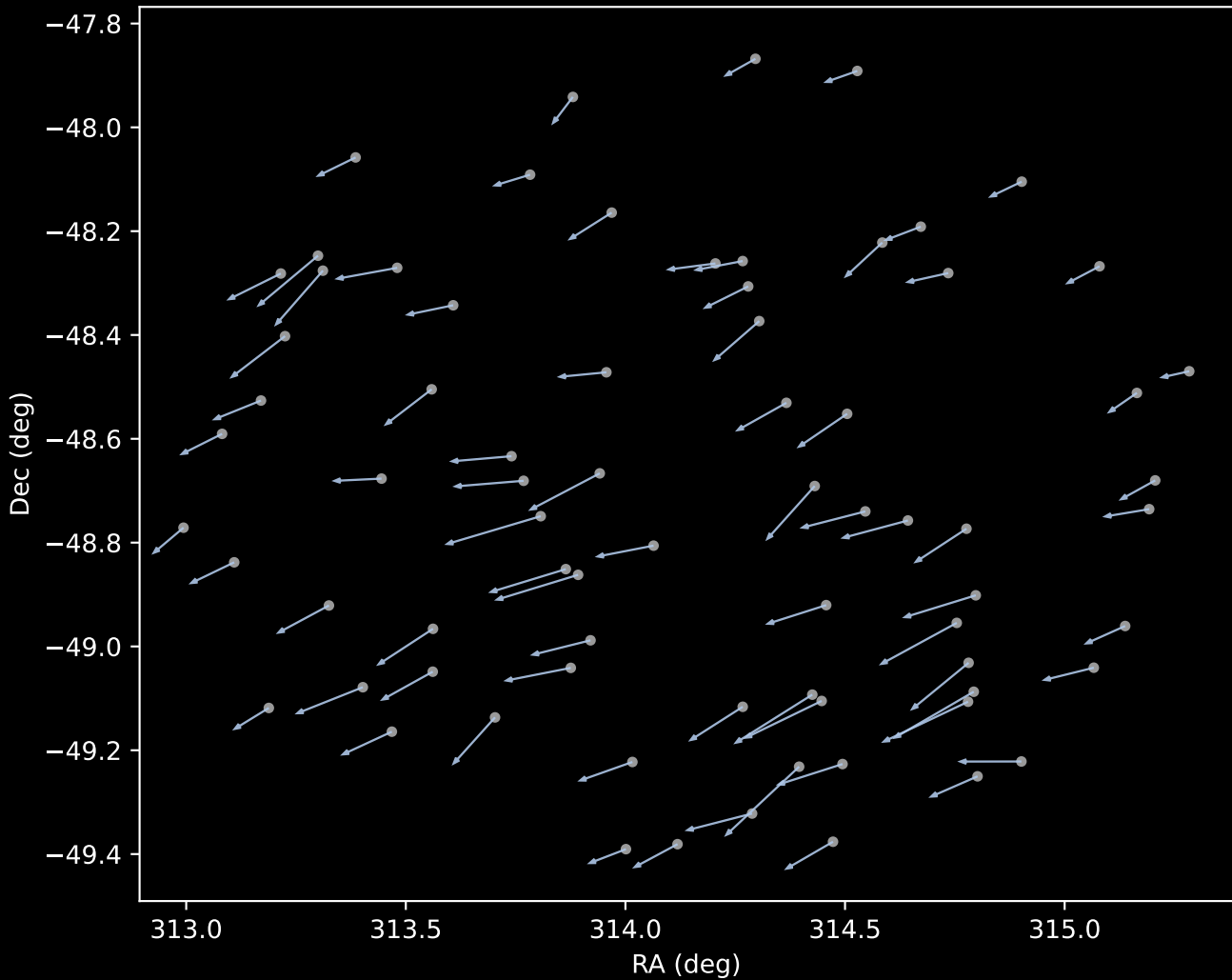
APOGEE DR17 Cluster 1 Proper Motion Vectors (n=74)
