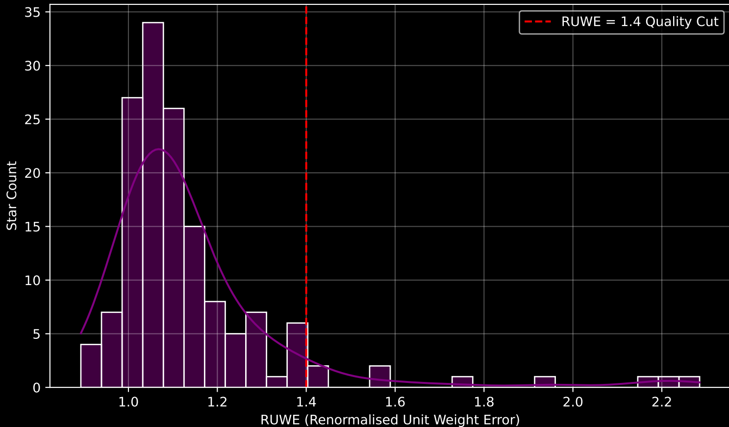
GAPOGEE DR17 Field [317+12] RUWE Distribution (n= 149)
